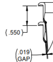
NESTING VIEW
