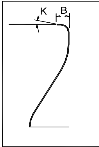
NECK DETAIL
