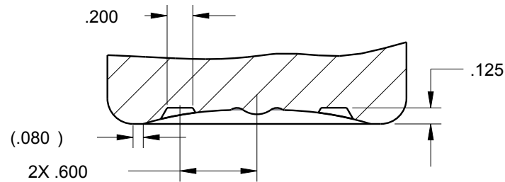
SECTION B-B SCALE 3/2
