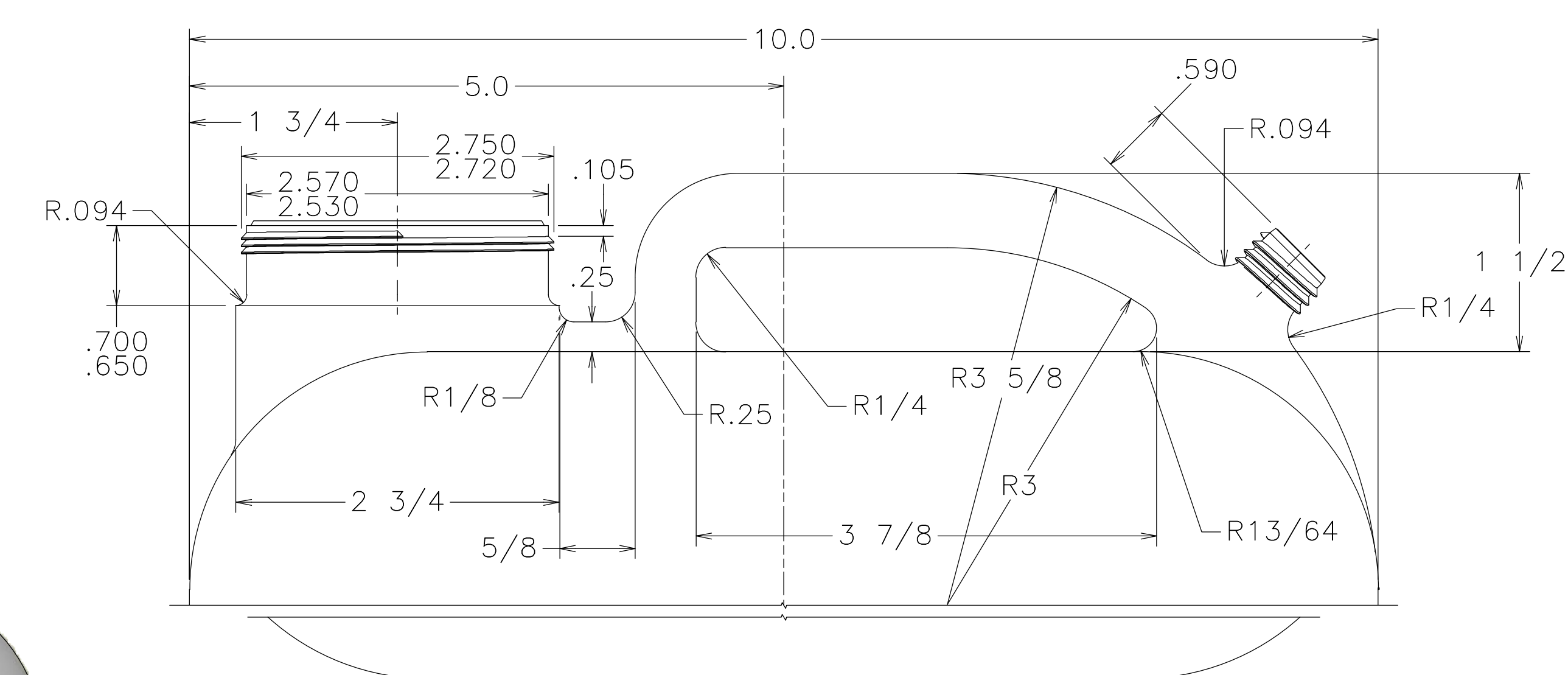
HANDLE AND 70mm RIEKE NECK DETAIL SCALE: 3 : 4 SECONDARY PRODUCT
