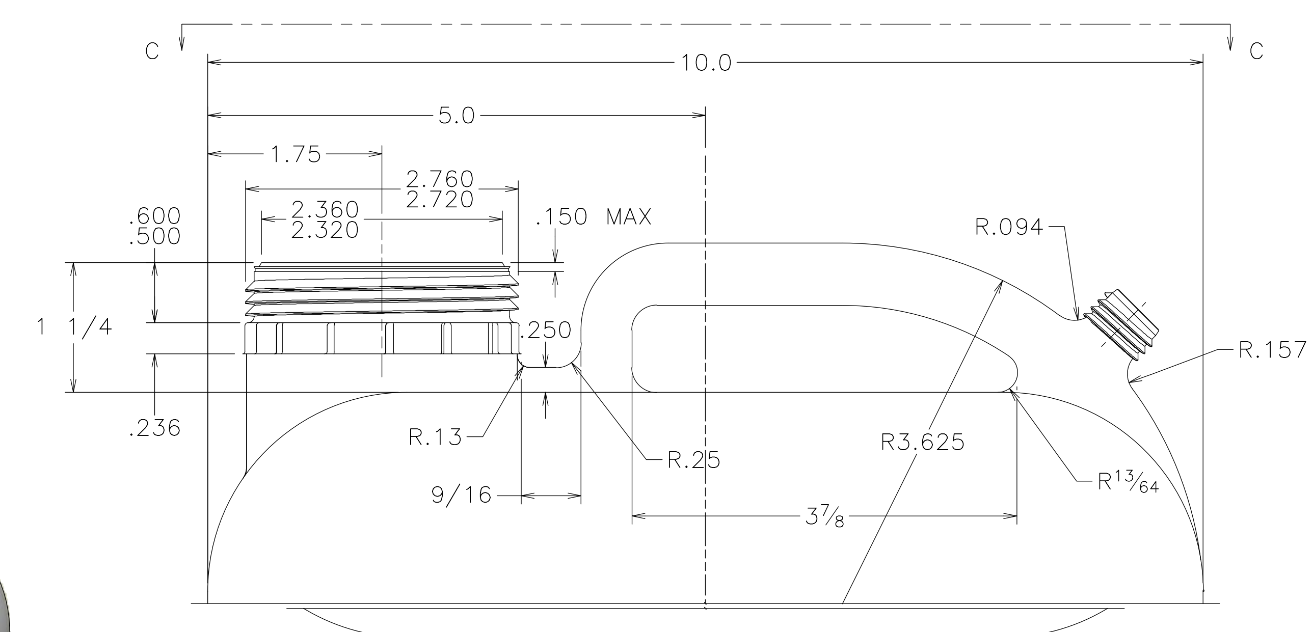
HANDLE AND 70mm TE THREAD RATCHET NECK DETAIL SCALE: 3 : 4 PRIMARY PRODUCT
