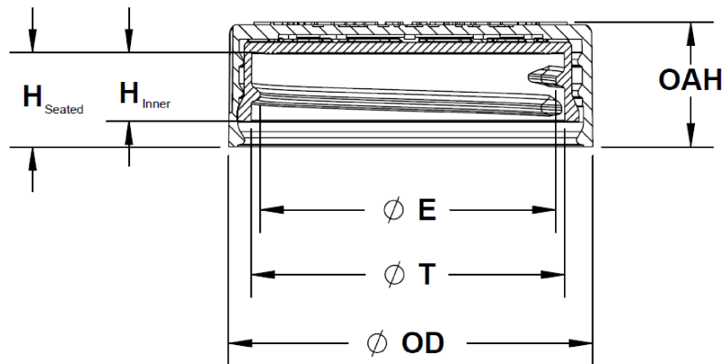
SECTION X-X SCALE 1 : 1
