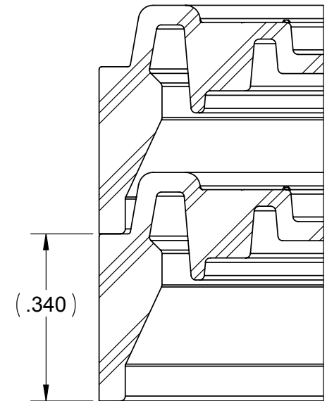
NESTING VIEW
