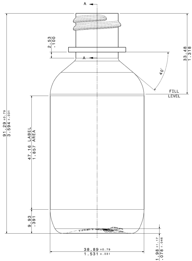
Front view Scale: 3:1
