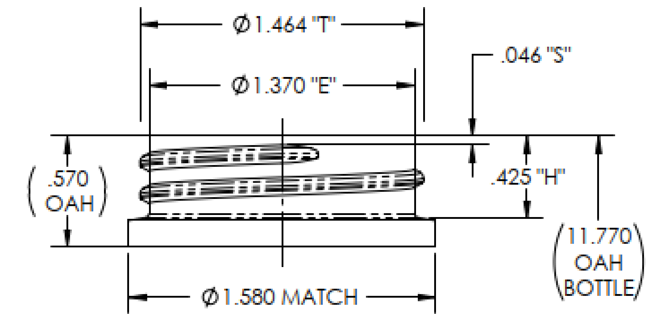
38mm SP-400 NECK FINISH DETAIL 3:2 SCALE
