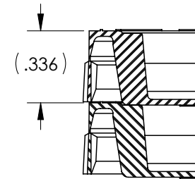
NESTING VIEW
